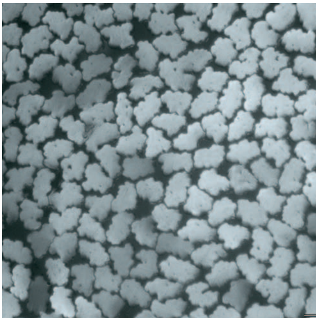
Cross section of Lenzing Viscose® 2.8 dtex / 30 mm dull
